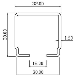
C30 Support Bracket
