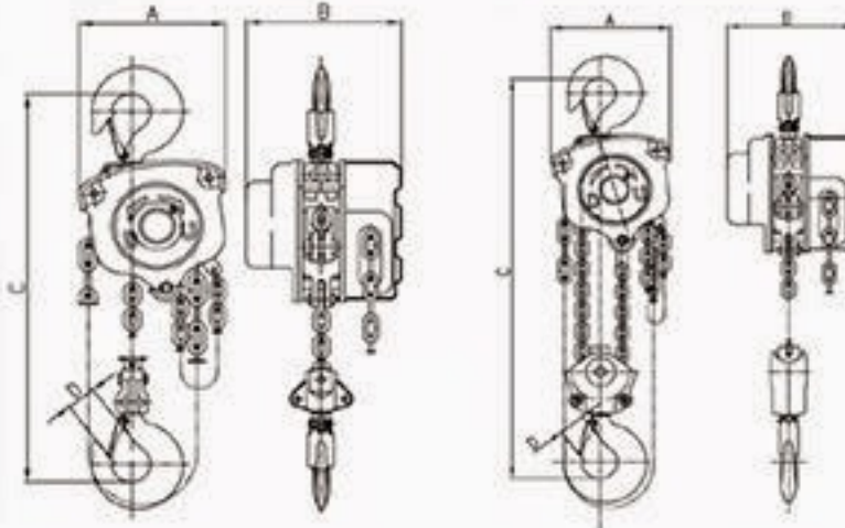
KT-C Chain Block (Single Chain)
